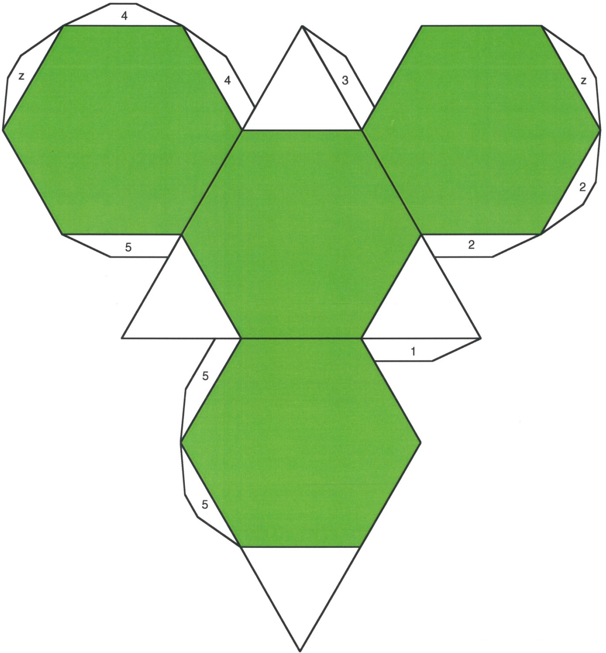
Truncated tetrahedron
