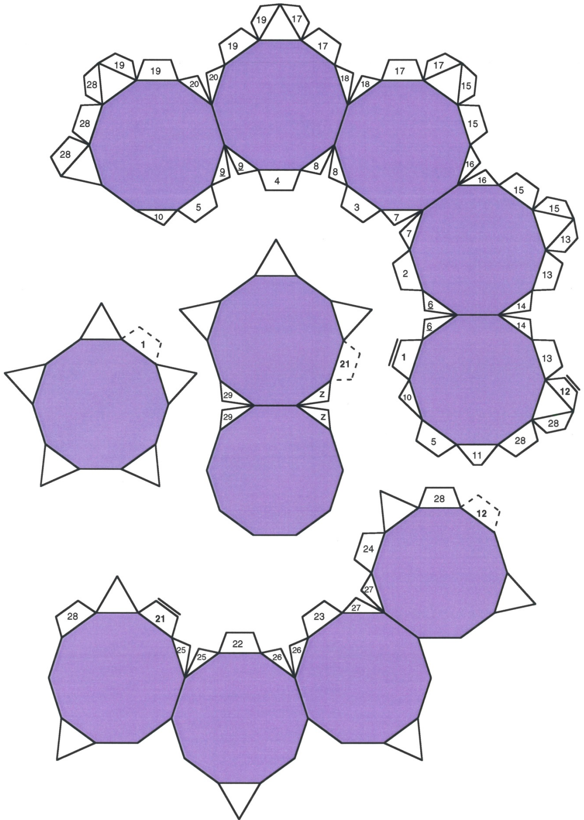
Truncated dodecahedron
