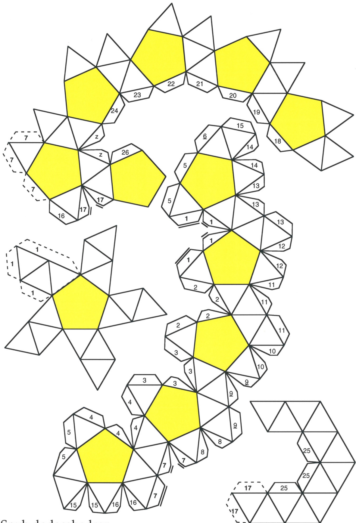
Snub dodecahedron
