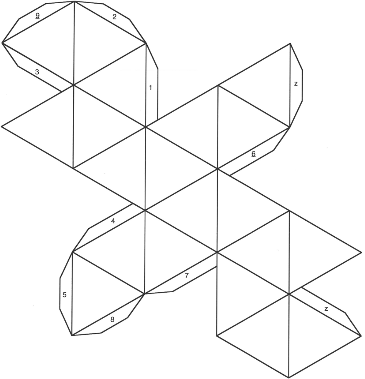
Icosahedron
