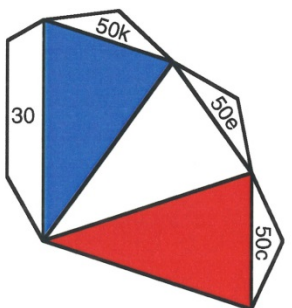
Great stellated dodecahedron - points
