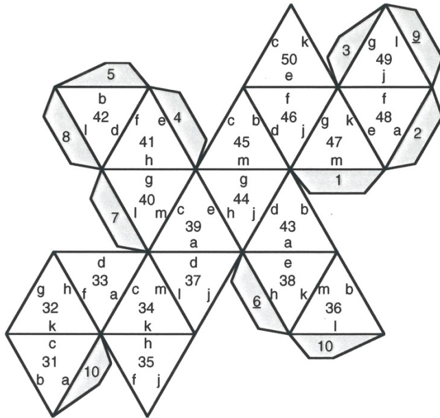
Great stellated dodecahedron - inner core
