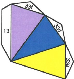
Great stellated dodecahedron - points
