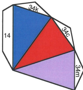
Great stellated dodecahedron - points
