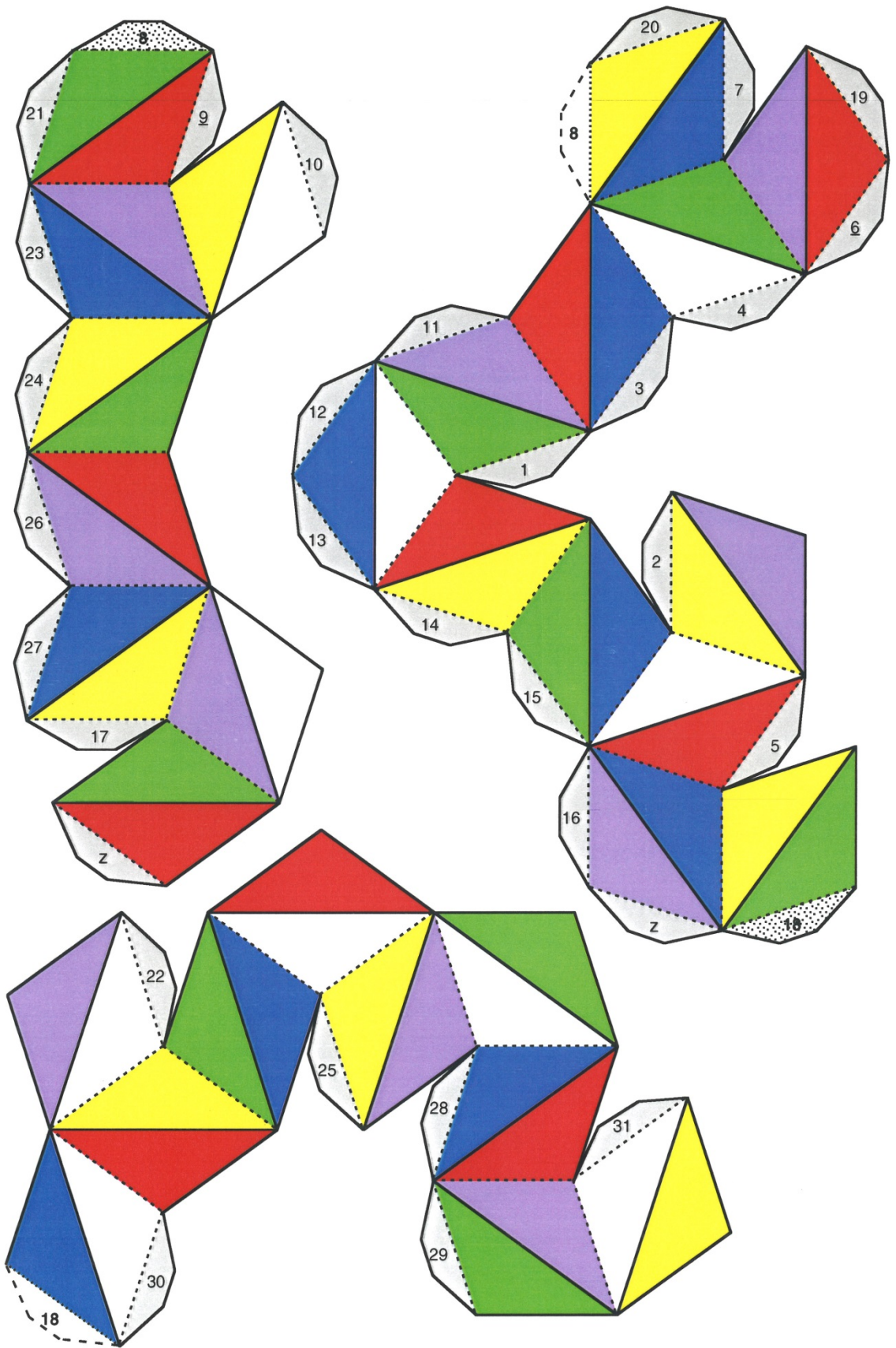
Great dodecahedron
