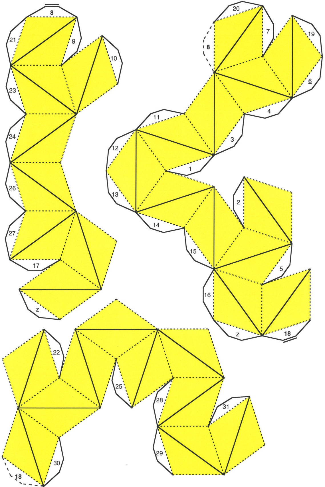
Great dodecahedron
