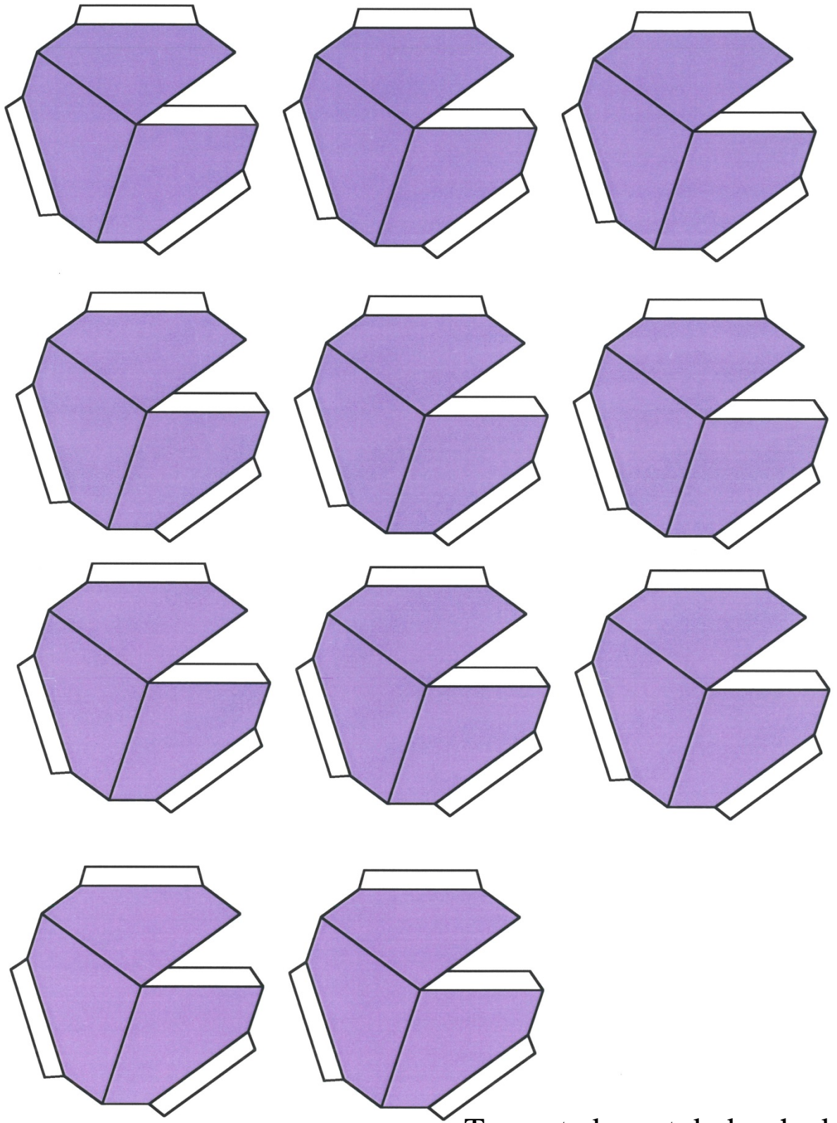
Truncated great dodecahedron Part 2
