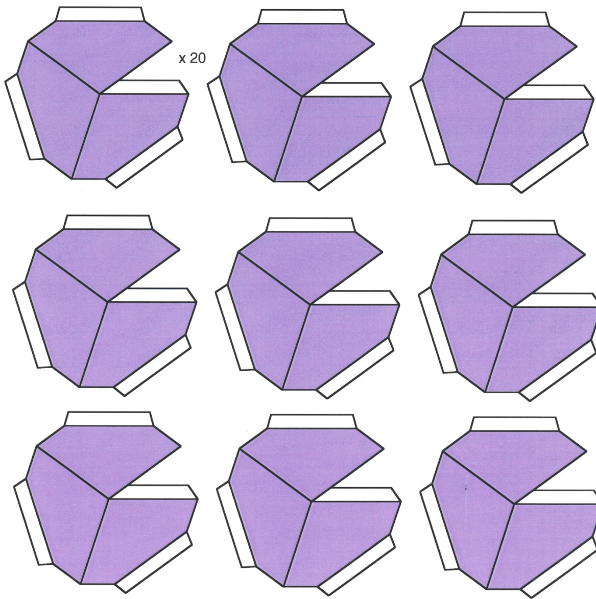
Truncated great dodecahedron Part 1
