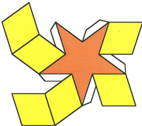
Dodecadodecahedron Part 1
