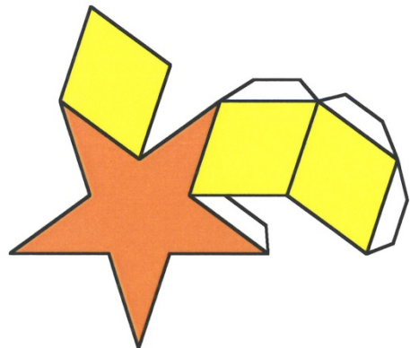
Dodecadodecahedron Part 2
