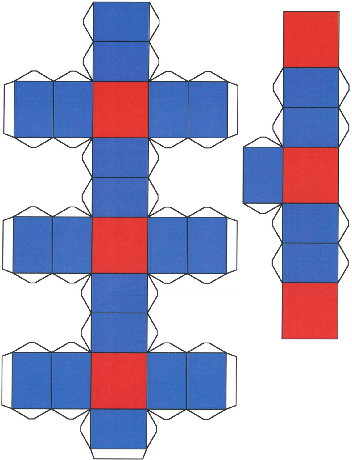
Small cuboctahedron Part 1
