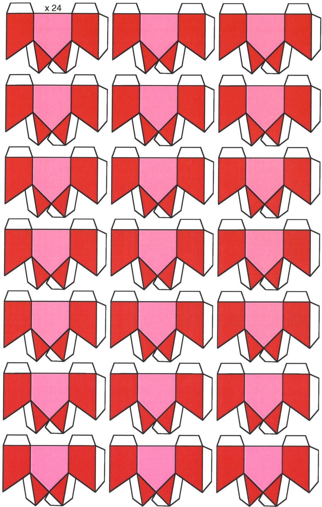
Quasirhombicuboctahedron Part 3
