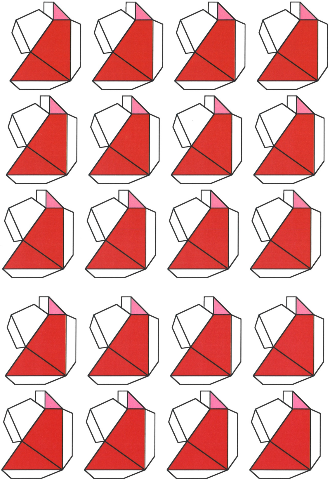
Quasirhombicuboctahedron Part 6
