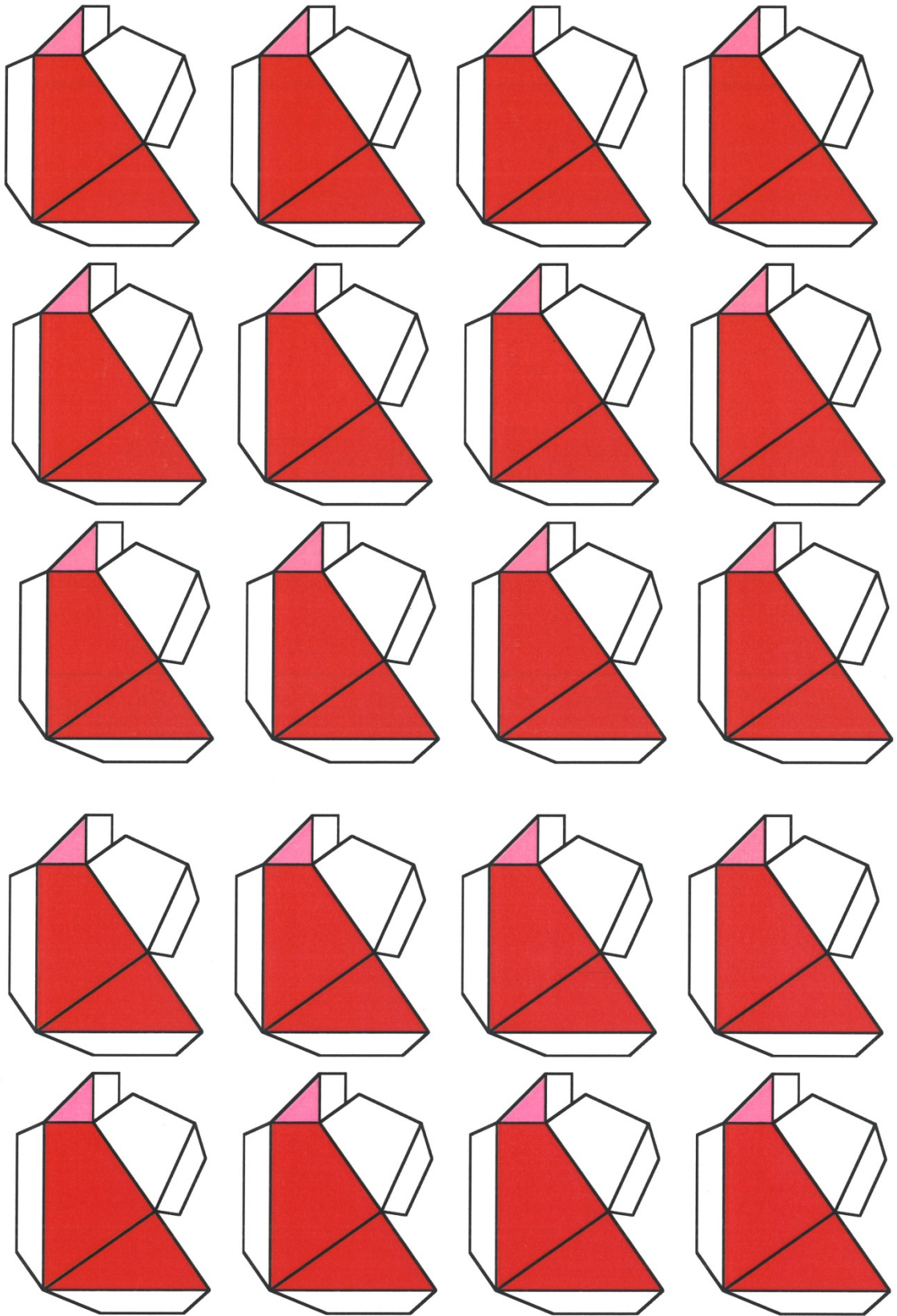
Quasirhombicuboctahedron Part 5
