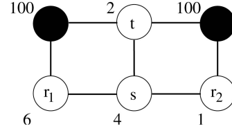
Fig. 3. A 2 \times 3 image where Algorithm 1 fails to produce an optimum path forest for f_{\text{abs}}^S , with \mathcal{S} = \{r_1, r_2\} . We have f_{\text{abs}}^S(s) = f_{\text{abs}}(\langle r_1, s \rangle) = 2 < f_{\text{abs}}(\langle r_2, s \rangle) = 3 , but f_{\text{abs}}^S(t) = f_{\text{abs}}(\langle r_2, s, t \rangle) = 3 < f_{\text{abs}}(\langle r_1, s, t \rangle) = 4 .
